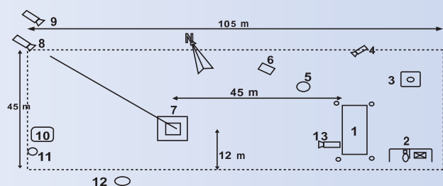
Control station
